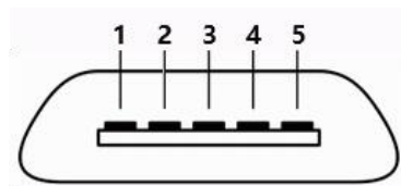
Micro-USB Female
