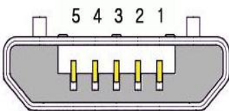
Micro-USB Male
